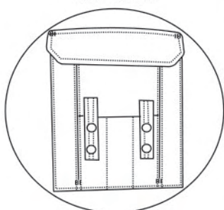
POCKET DETAIL
